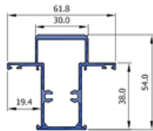
Mullion 54 38 CW3821
