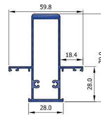
Mullion 70 28 CW2822
