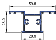
Mullion 28 CW2842
