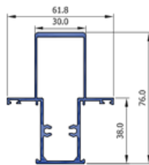
Mullion 76 38 CW3822
