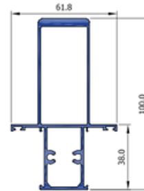
Mullion 100 38 CW3823
