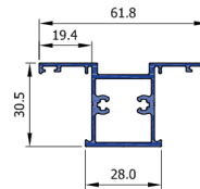
Mullion 30.5 CW3042
