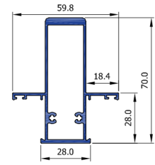
Mullion 70 28 CW2822
