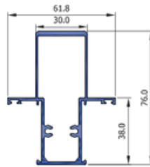
Mullion 76 38 CW3822
