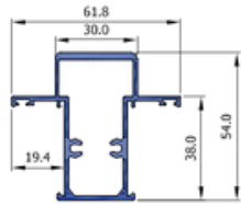
Mullion 54 38 CW3821
