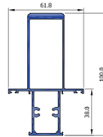
Mullion 100 38 CW3823
