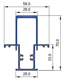
Mullion 70 34 SCW3422
