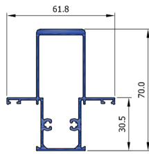
Mullion 70 30.5 CW3022
