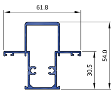
Mullion 54 30.5 CW3021
