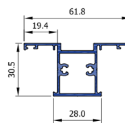
Mullion 30.5 CW3042
