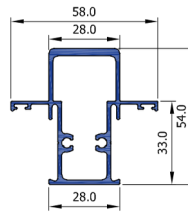
Mullion 54 34 SCW3421
