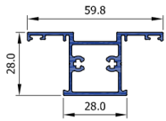
Mullion 28 CW2842
