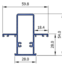
Mullion 54 28 CW2821
