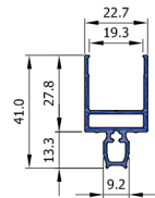
Patio Slider Double Glazing Adaptor
