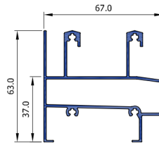
Zenith Horizontal Slider Double Cill
