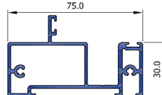
Folding Door Head FD02
