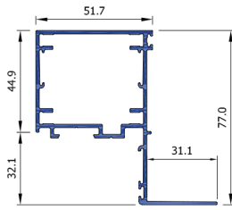
Double Flush Glazed Sash SF44605
