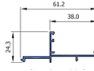
Adaptor Shopfront 38 Casement SF44165
