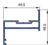
Shopfront Sash SF44411
