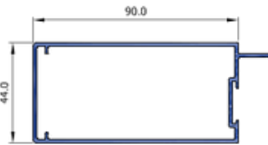
R9 Door Stile 90 (R1 90) SF44040
