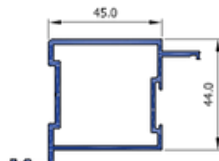
R12SP (L& W) Door Stile 45mm SF44012
