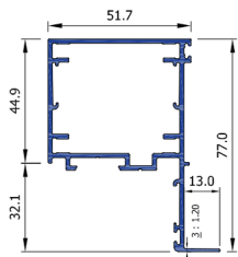
Single Flush Glazed Sash SF44604
