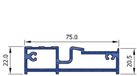
Folding Door Internal Cill FD11
