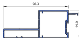
Maglock Stile Open SF44043
