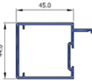
R1 Door Stile 45mm SF44010
