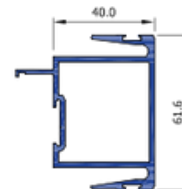
Double Fixed Interlocked 40mm HDS016DF
