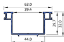
HDS Double Threshold Channel HDS041
