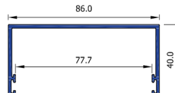
Compensating Channel 86x40mm SF44991
