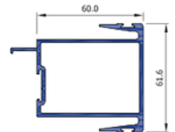
Double Fixed Interlocked 60mm HDS027DF
