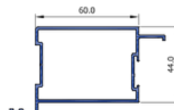
R11SP (L& W) Door Stile 60 (R12SP 60) SF44022
