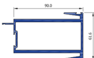
Double Fixed Interlocked 90mm HDS018DF
