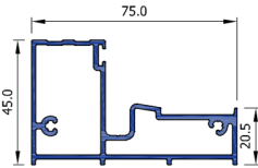
Folding Door Cill FD01
