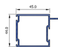
R3 (W) Door Stile 45mm SF44011
