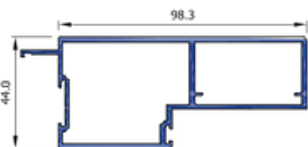
Maglock Stile Fixed SF44044
