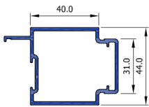
HDS Meeting Stile 40 HDS012
