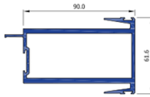
Double Fixed Interlocker 90mm HDS018DF
