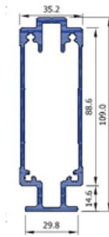
Adaptor Stiffener HDS032
