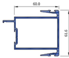
Double Fixed Interlocker 40mm HDS027DF
