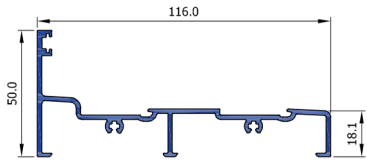
HDS Double Cill HDS004
