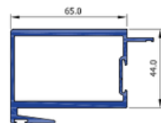
HDS Fixed Interlocker 65 HDS037F
