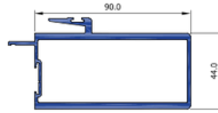
HDS Sliding Interlocker 90 HDS018S
