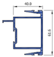
Double Fixed Interlocker 40mm HDS016DF
