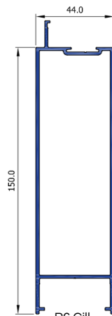
R6 Cill Rail 150mm SF44018
