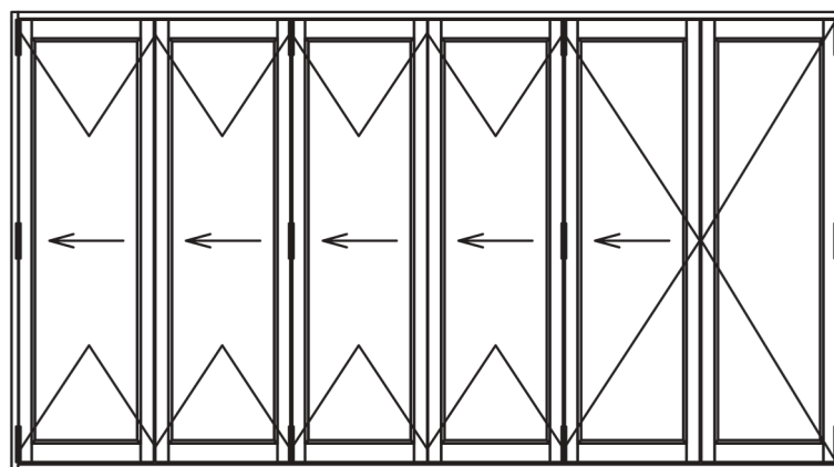
5 Panel (with Hinged Door)
