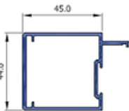
R1 Door Stile 45mm SF44010
