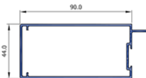
R9 Door Stile 90 (R1 90) SF44040
