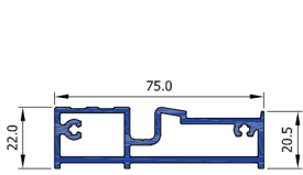
Folding Door Internal Cill FD11
