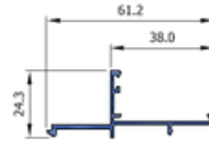
Adaptor Shopfront 38 Casement SF44165
