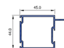
R3 (W) Door Stile 45mm SF44011
