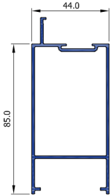
R4 Head/Cill Rail 85mm SF44014
