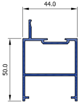
Folding Door Internal Cill FD11
