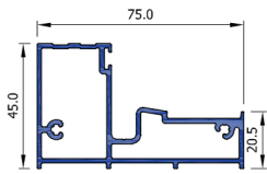
Folding Door Cill FD01
