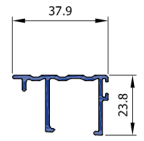
Patio Slider Cill Cover
